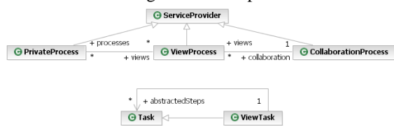
Fig. 6: PIM4SOA extension
