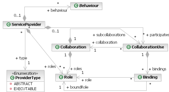
Fig. 1: PIM4SOA: structure
