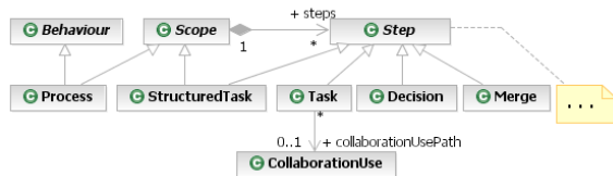
Fig. 2: PIM4SOA: behaviour
