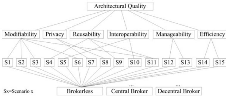
Fig. 7 AHP decomposition tree for CBP evaluation model
