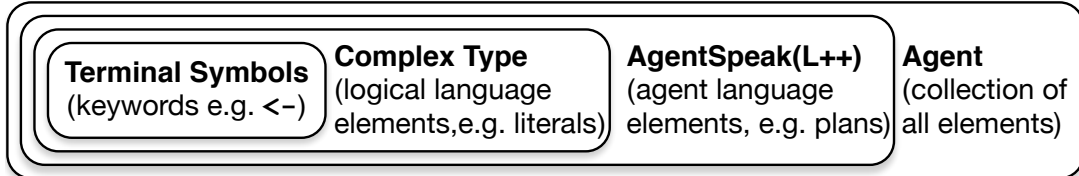
Figure 1: Modular Grammar Structure
