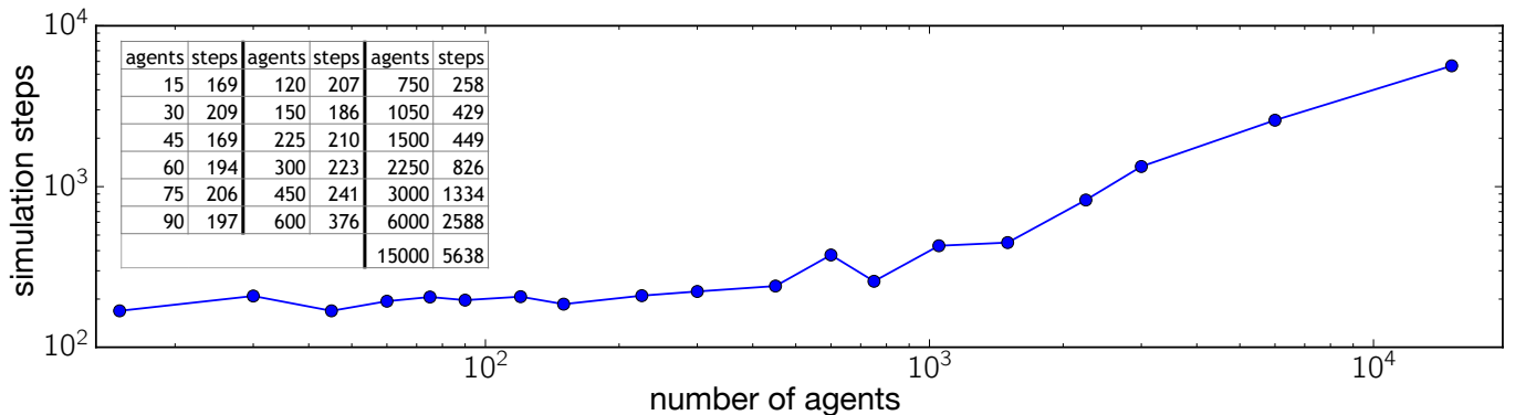
Figure 2: Number of agents plotted against cycles until all agents left the scenario.
